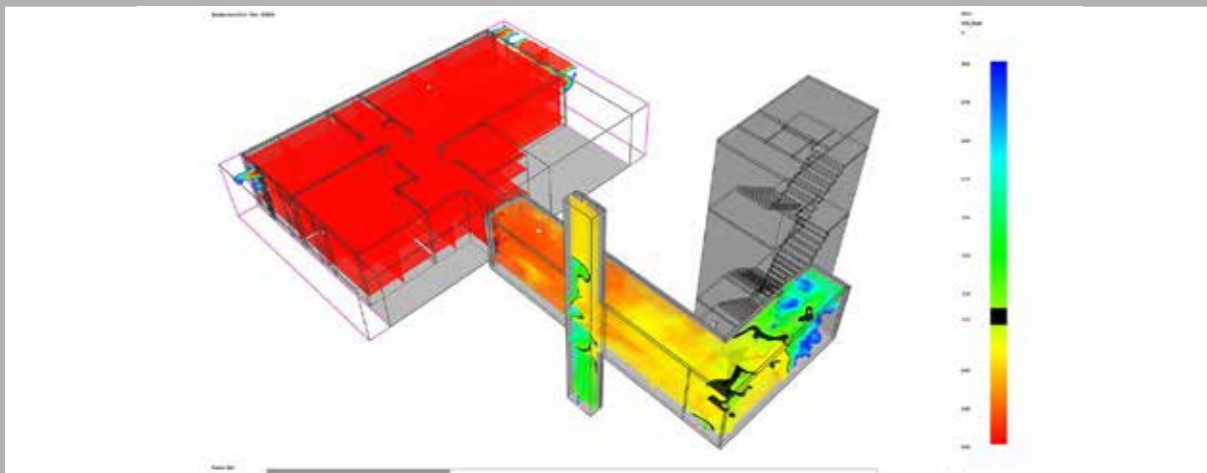
We use computational fluid dynamics models to measure the clearance of smoke from our ventilation systems.
